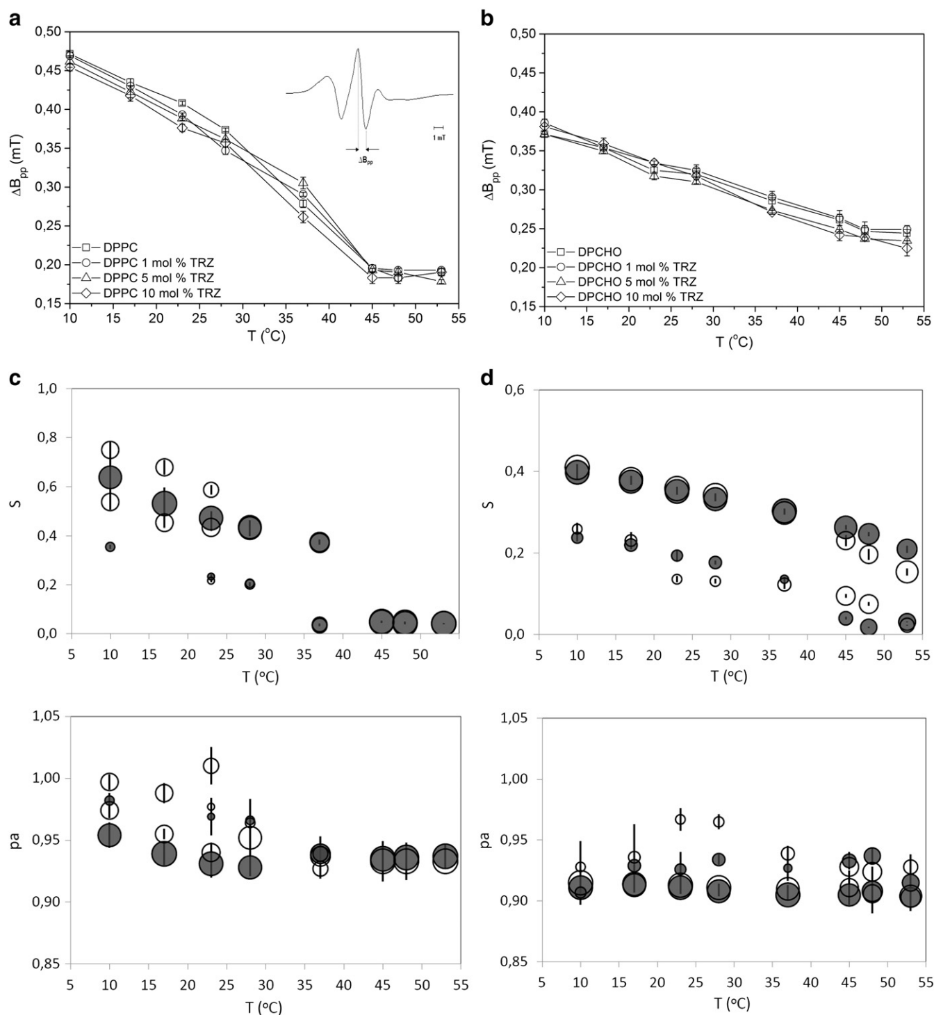
Fig. 4. Temperature dependence of \Delta B_{pp} of 16-DS in a) pure, b) 30 mol% of CHO incorporated DPPC MLVs at various concentrations of TRZ. Temperature dependence of 10 mol% TRZ induced changes in the order parameters (S) and polarity correction factor (pa) of 16-DS in c) pure, d) 30 mol% CHO incorporated DPPC MLVs. Gray and white circles point out pure and 10 mol% TRZ incorporated samples respectively. Diameter of circles denotes the proportion of spin probe in different domain types. Bars indicate second moment in the distribution of values obtained from the GHOST condensation technique.
