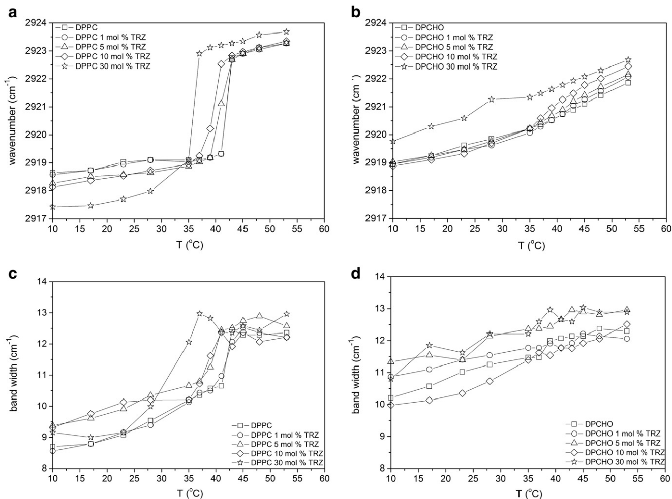
Fig. 7. Temperature dependence of the frequency and bandwidths of CH 2 asymmetric stretching bands of a–c) pure, b–d) CHO incorporated DPPC MLVs in the absence and presence of various concentrations of TRZ.
