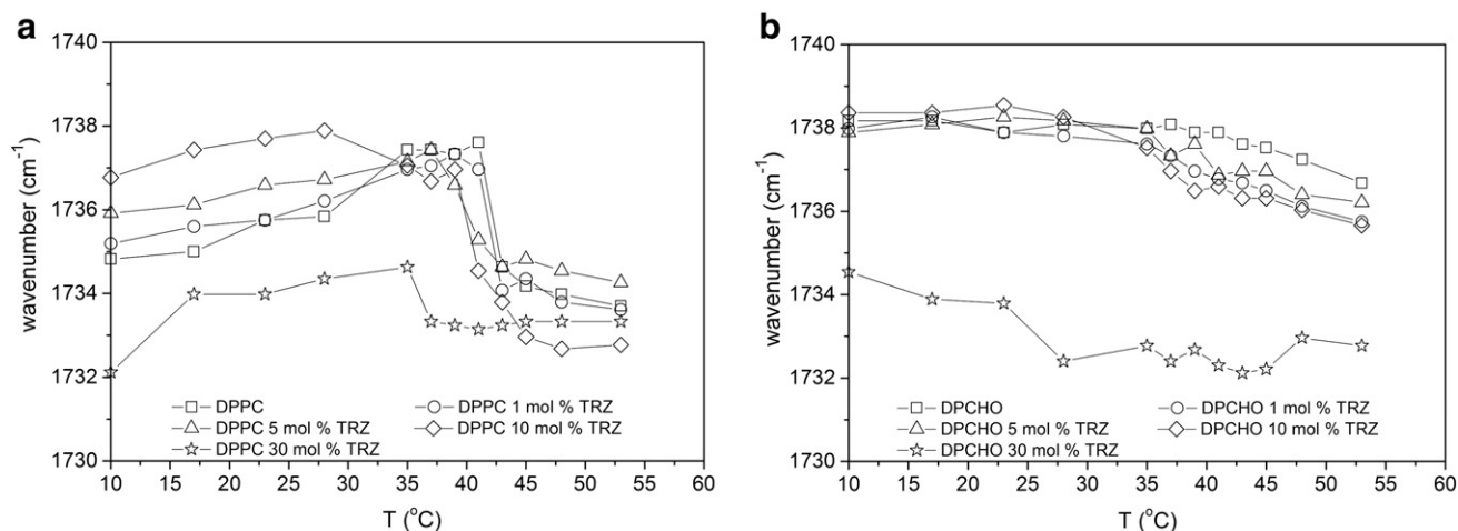
Fig. 8. Temperature dependence of the frequency changes at the C=O stretching band for a) pure and b) CHO incorporated DPPC MLVs in the absence and presence of 1, 5, 10, 30 mol% TRZ.
